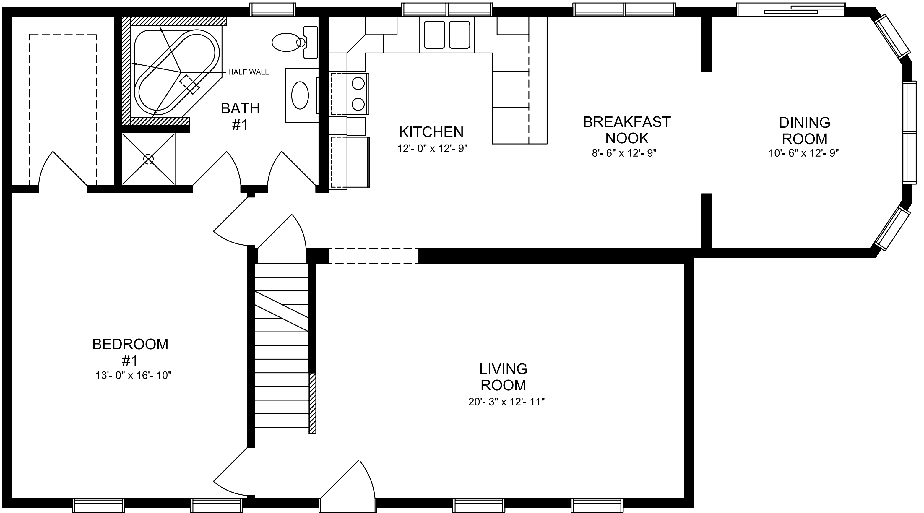
CUMBERLAND 27'- 6" X 38'/50'
