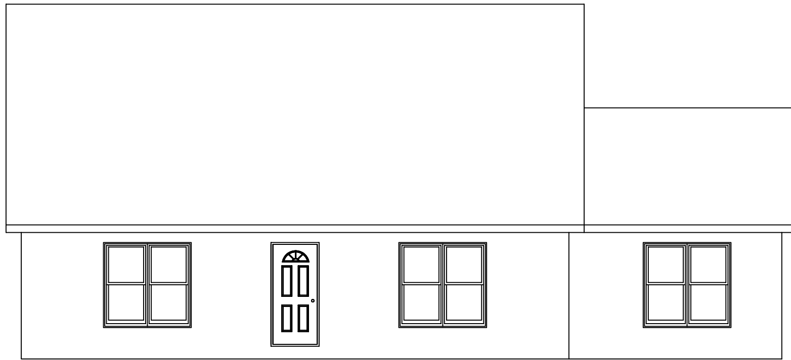
FRONT ELEVATION
