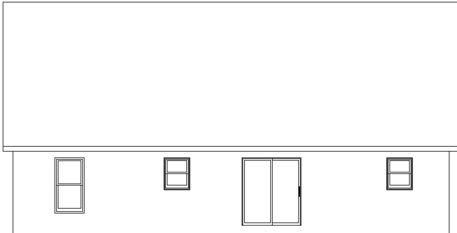
REAR ELEVATION
