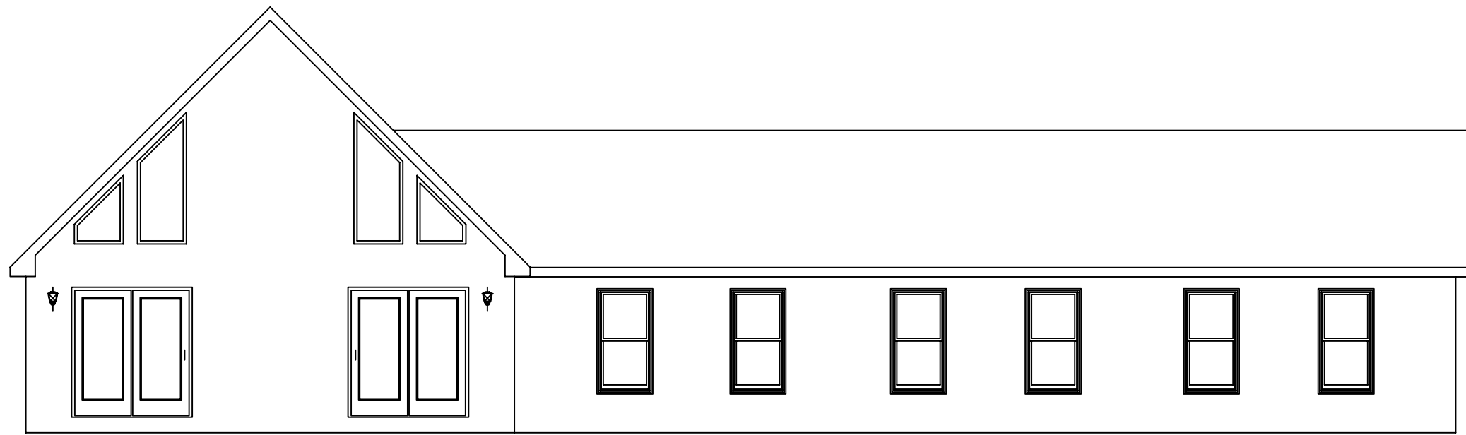
FRONT ELEVATION
