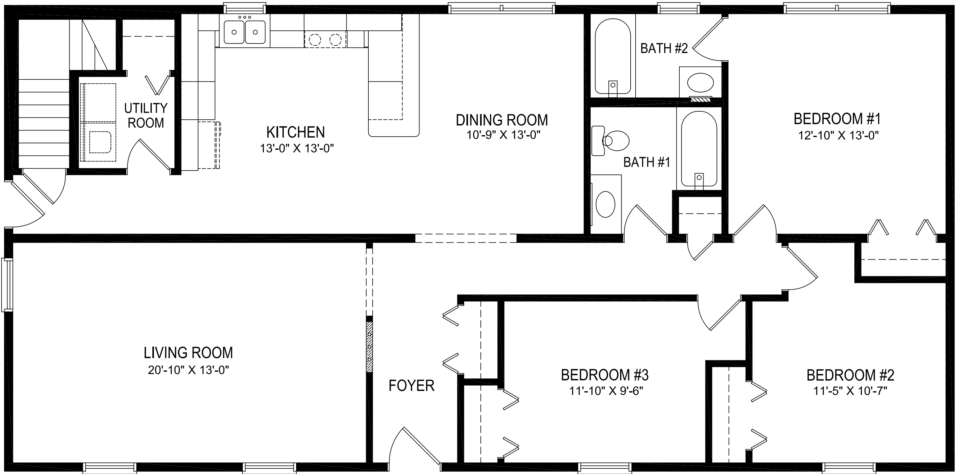
MILLERSVILLE 27'-6" X 56'-0"
