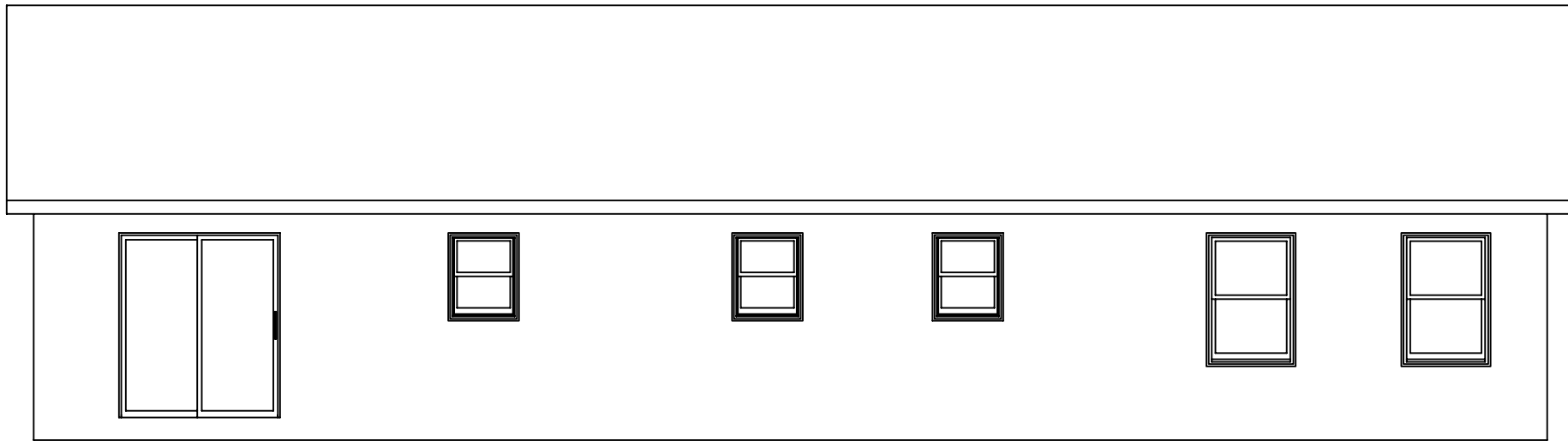
REAR ELEVATION
