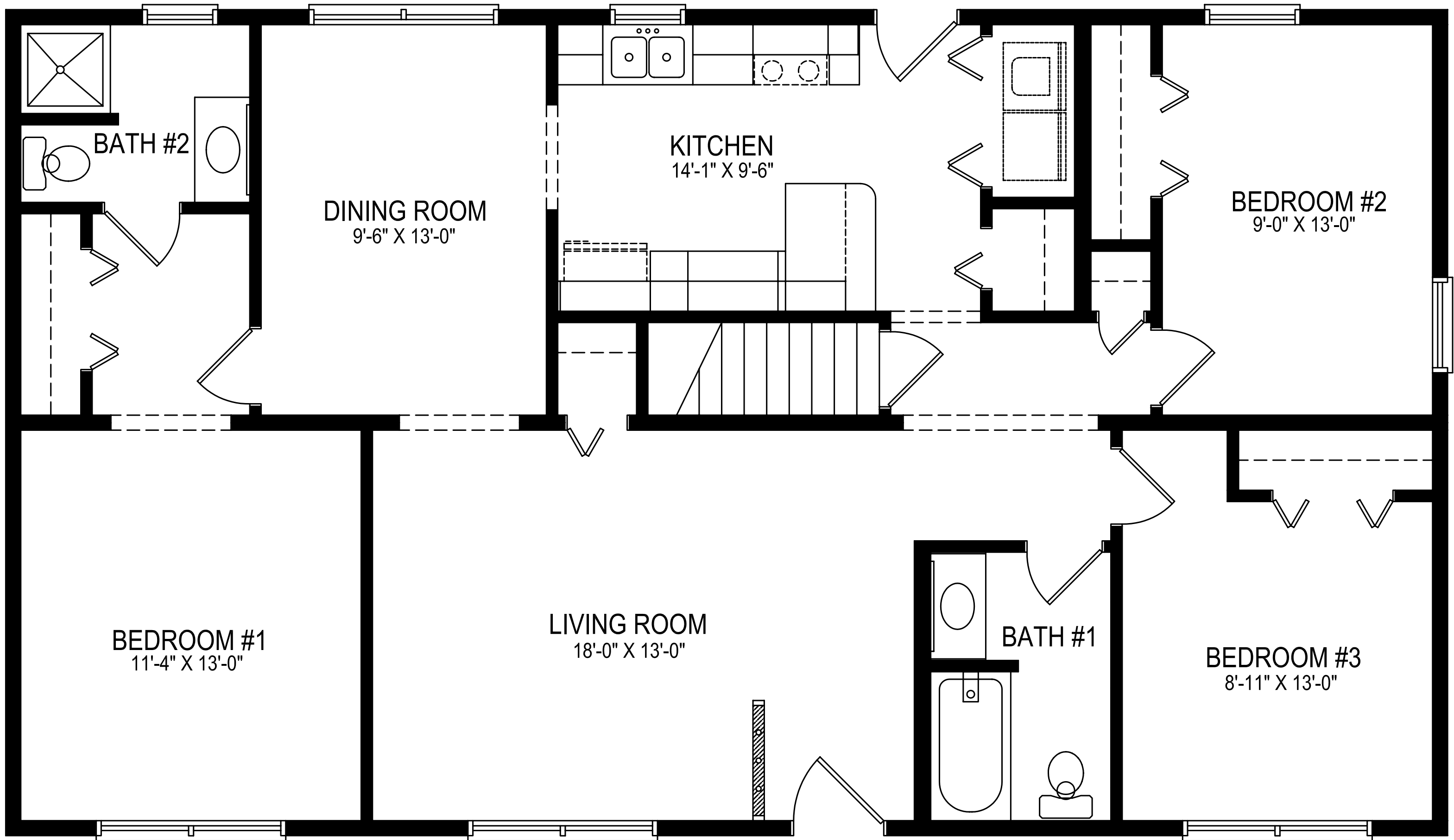
WARMINSTER 27'-6" X 48'-0"
