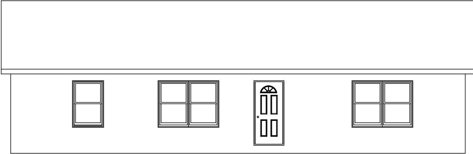
FRONT ELEVATION
