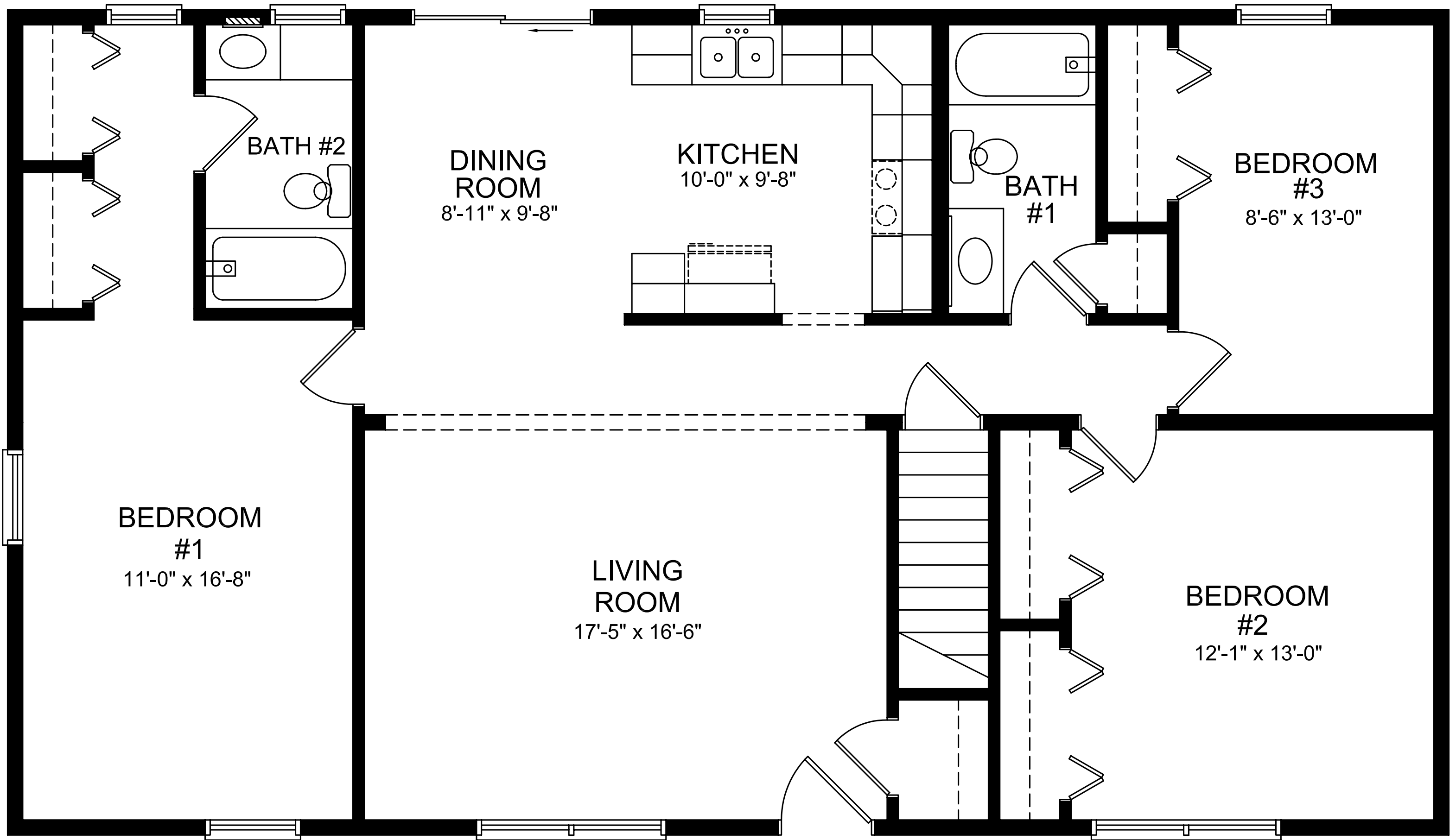
WATERTOWN II 27'-6" x 48'
