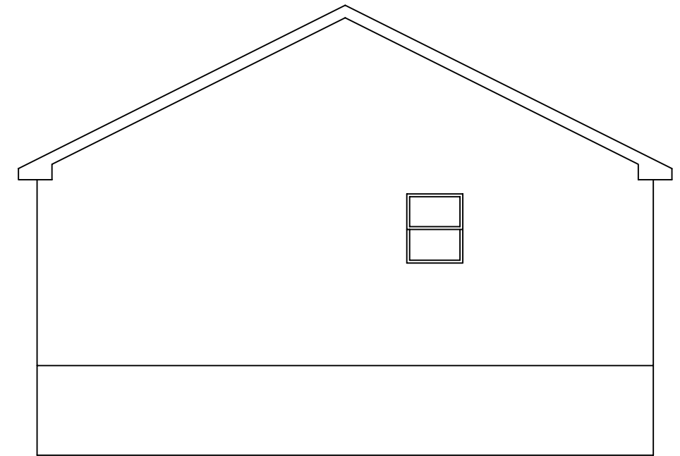
LEFT ELEVATION
