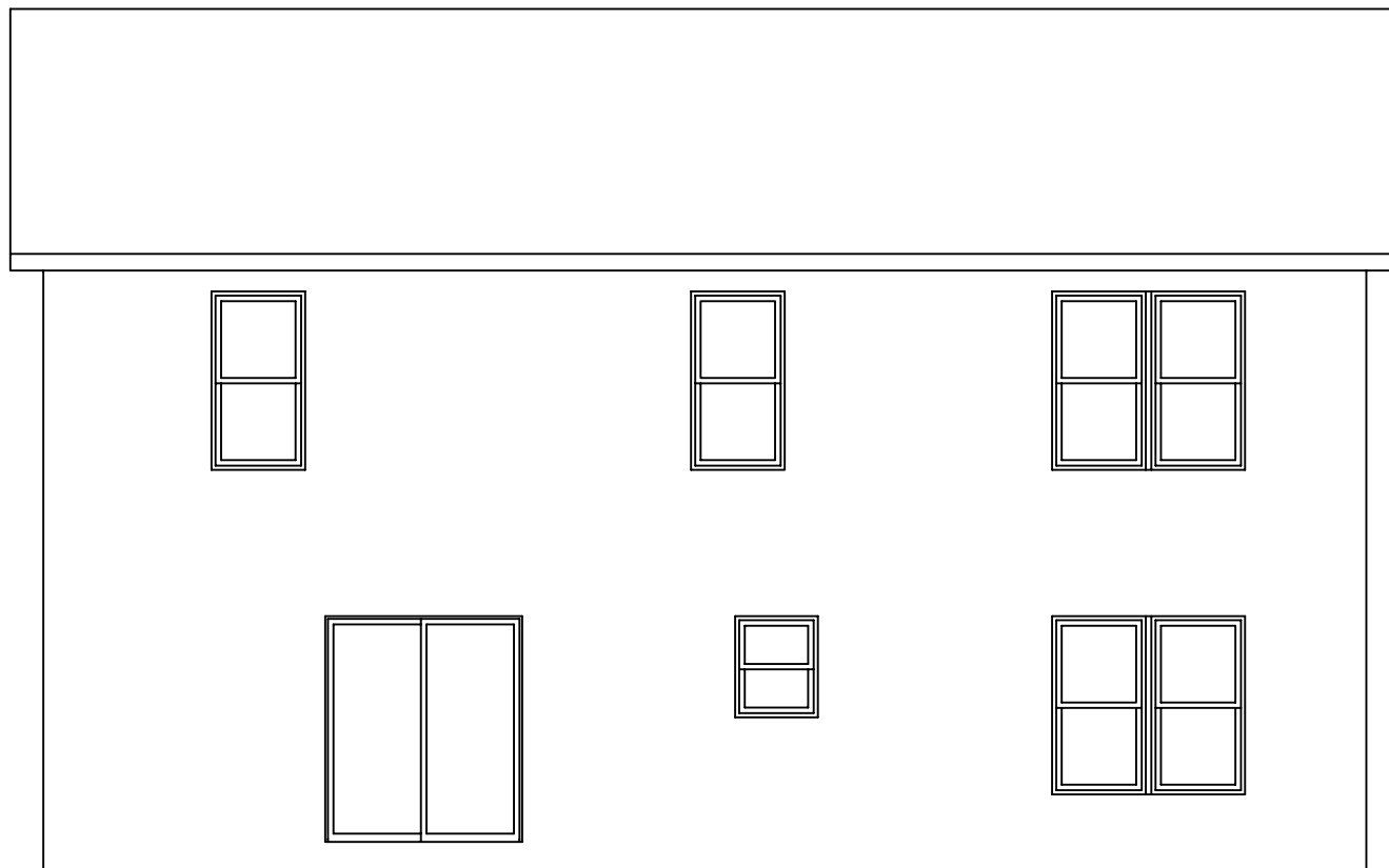
REAR ELEVATION
