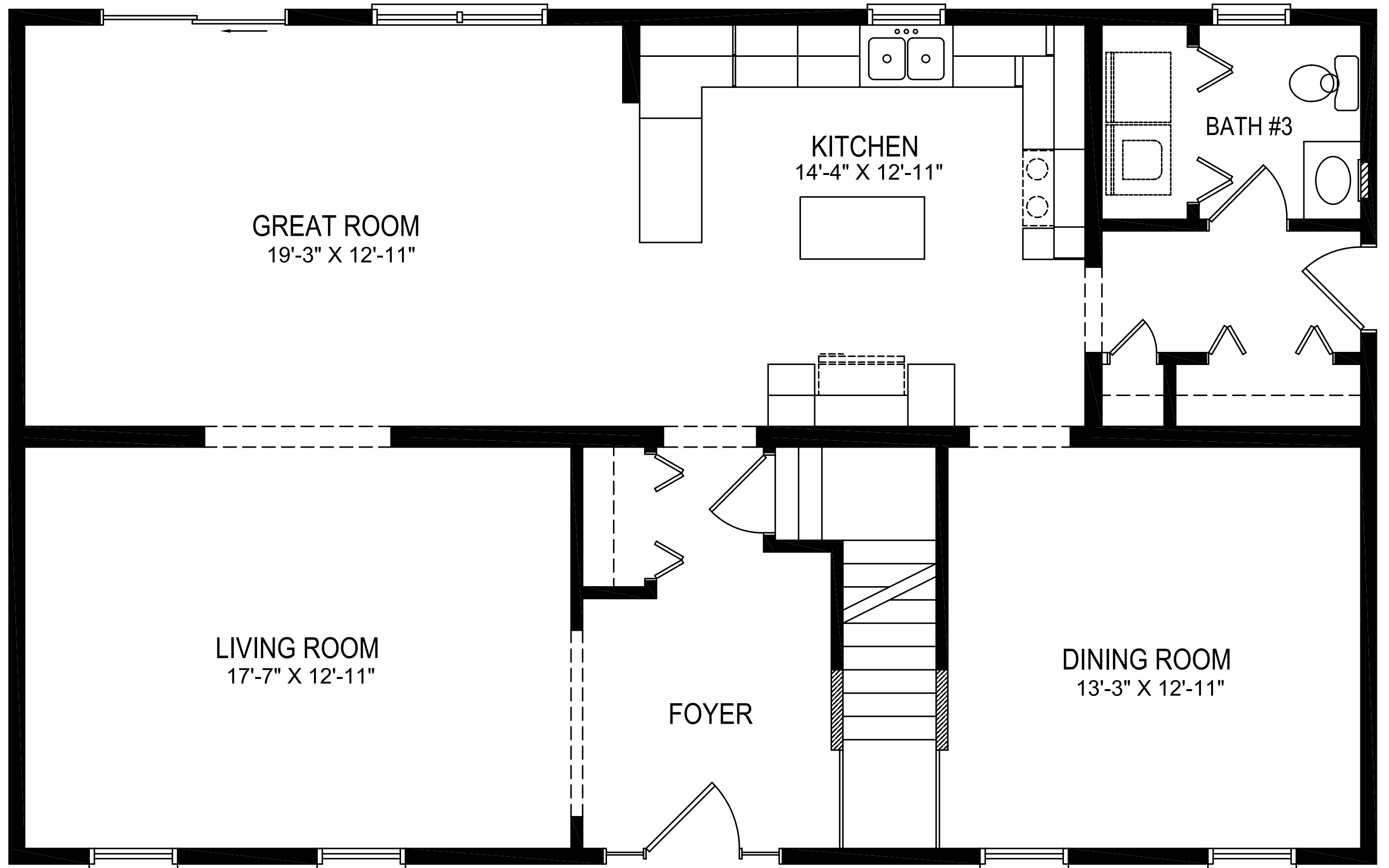
MIDDLE HOPE 27'-6" X 44'-0"
