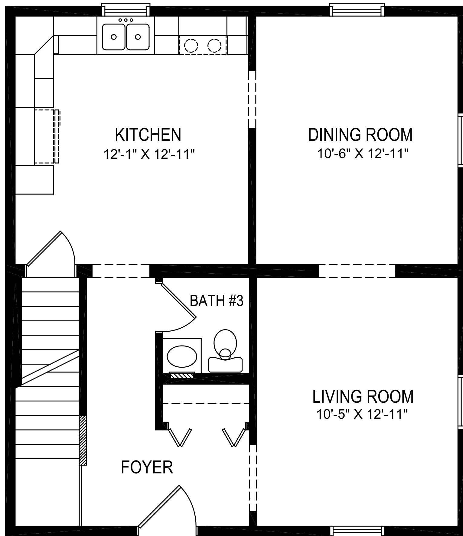
NEW PALTZ 27'-6" X 24'
