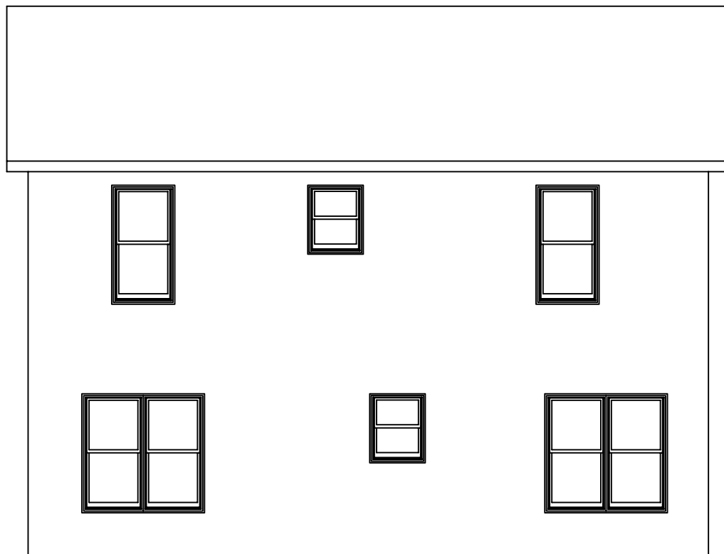
REAR ELEVATION
