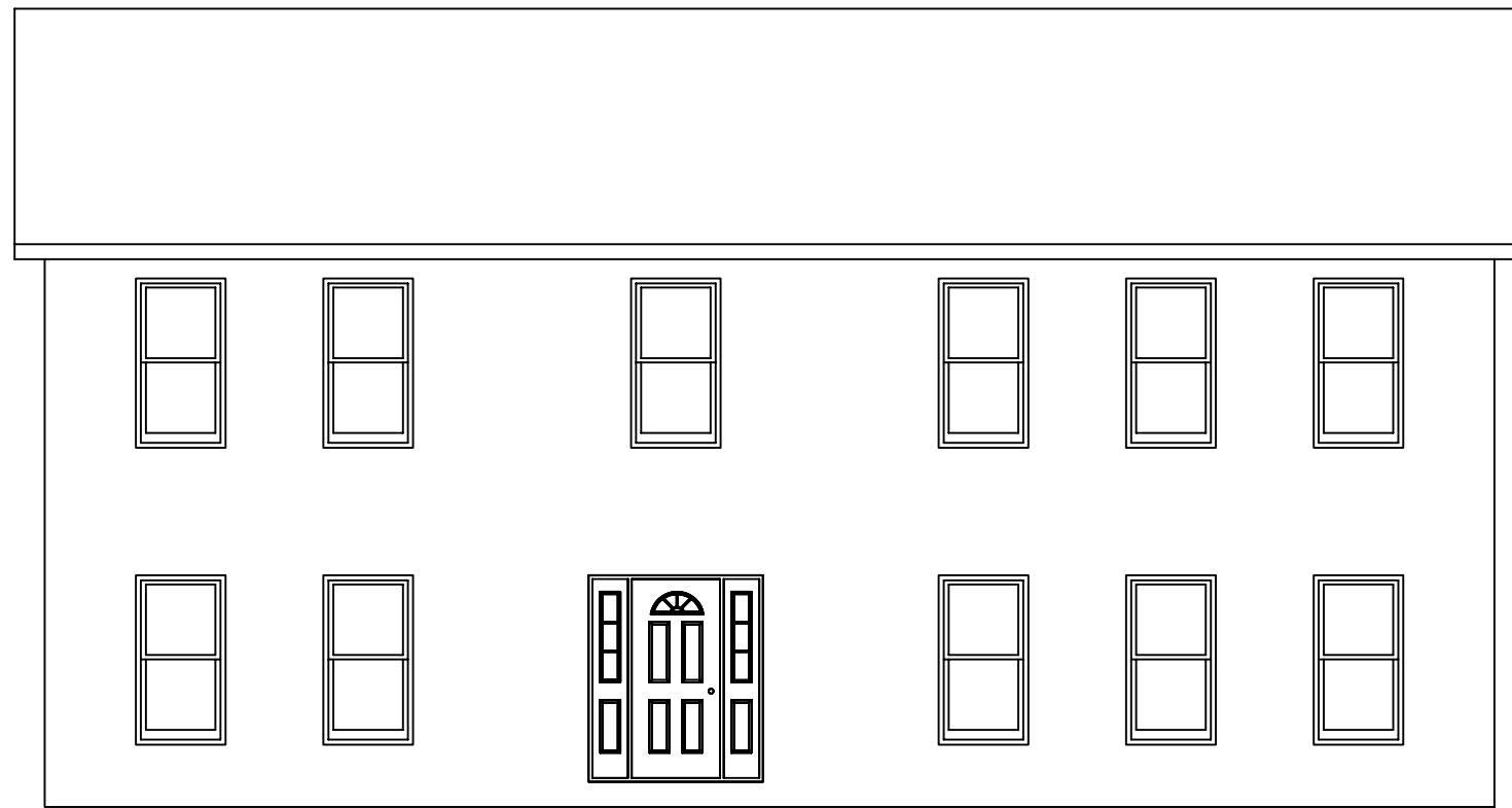
FRONT ELEVATION
