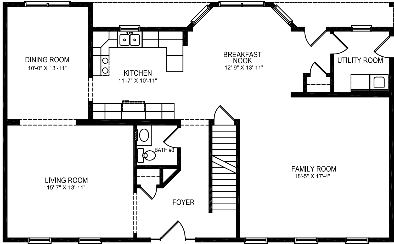
OAKDALE 29'-6" X 48'
