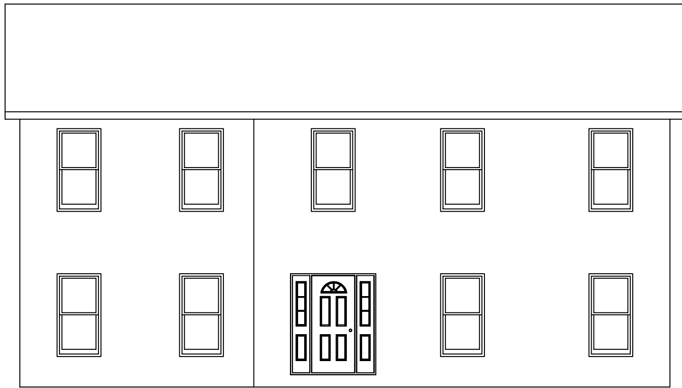
FRONT ELEVATION
