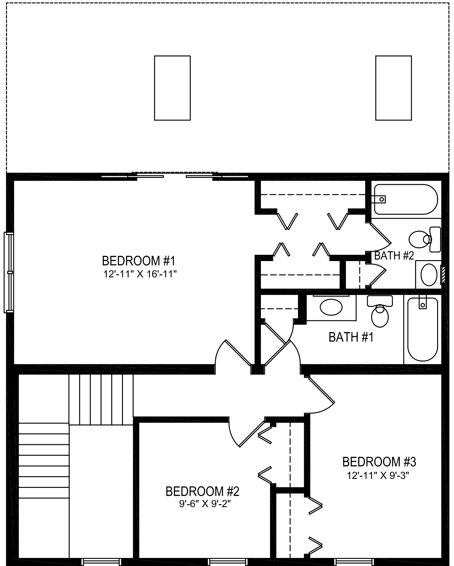
ROCKPORT 39'-5" X 31'-0"
