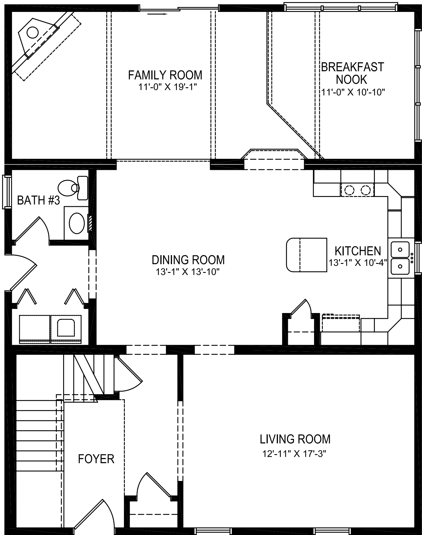
ROCKPORT 39'-5" X 31'-0"
